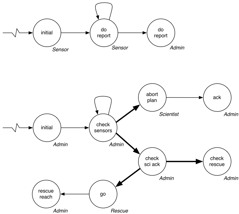
Fig. 13. Event graph of the sensor network model. Notice there are two events that start the system.
