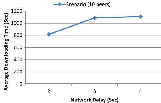
(c) Average downloading time for different network delays.
