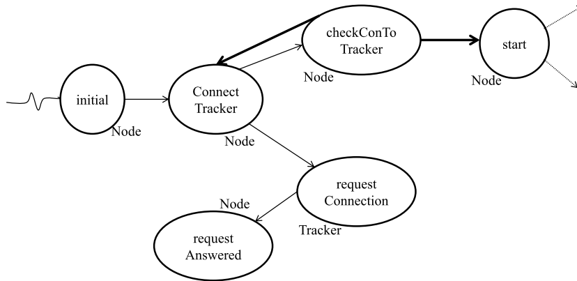
Fig. 14. Event graph of connecting a peer to the tracker.
