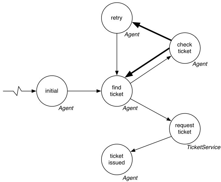
Fig. 12. Event graph of the ticket service model.
