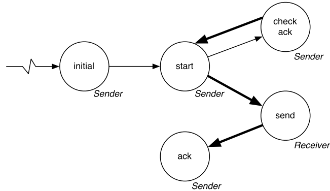
Fig. 11. Event graph of the simple communication protocol model.
