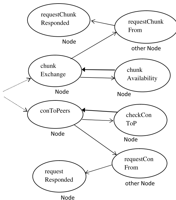
Fig. 15. Event graph of connecting to the peers and downloading chunks from them.
